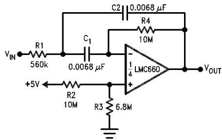
10 Hz Bandpass Filter
